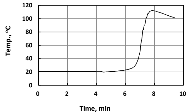
Typical Exotherm Curve for DEVCON® MA2060 in 10 gm Mass at 23 °C (73 °F)
