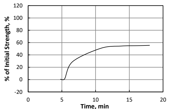
Tensile Shear Strength Development on Al6061
